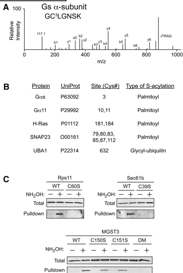
Fig. 3. Identification of S -acylation sites by acyl-RAC coupled with mass spectrometry. A: Representative MS/MS spectrum of the N-terminal peptide from the heterotrimeric GTPase G \alpha s containing Cys 3 , the known site of S -palmitoylation. The 117 amu peak corresponds to the reporter ion from the NH 2 OH+ sample, whereas the 114 amu peak (control) was not detected. B: Representative list of known S -acylated sites identified by MS-coupled acyl-RAC (see supplementary Table I for the complete listing of sites identified). C: Validation of MS data by transfection of HEK293 cells with putative S -acylated proteins followed by acyl-RAC and immunoblotting for the specified individual proteins. In each case, the identified sites of S -acylation were mutated to serine as noted. For MGST3, the identified peptide contained two Cys residues (Cys 150 and Cys 151 ); therefore, both single and double mutants (DM) were subjected to acyl-RAC.
